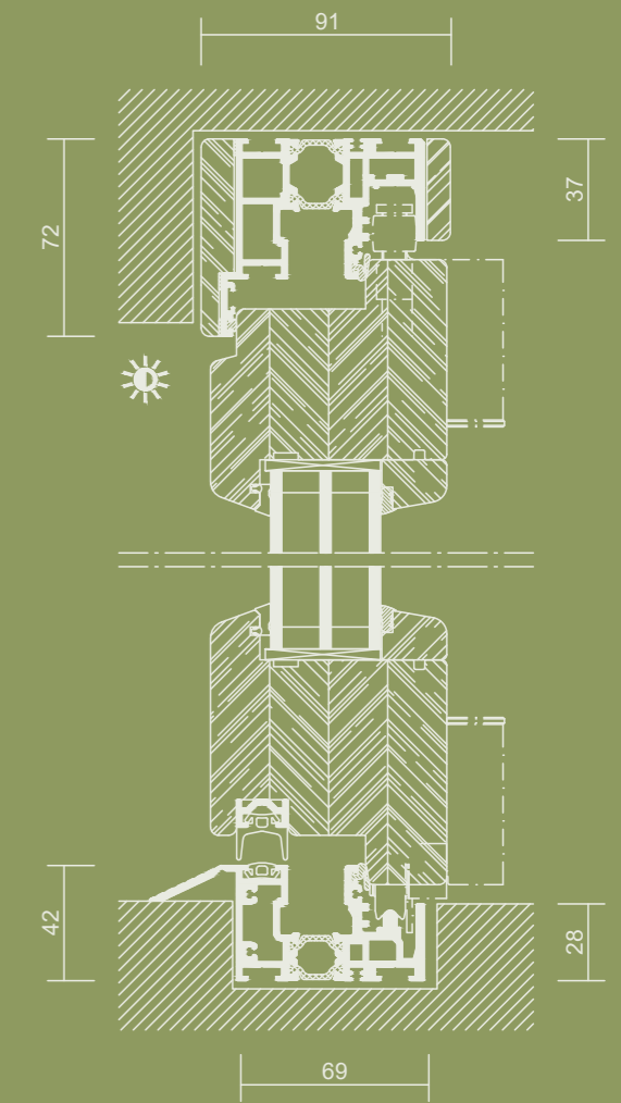
Vertical section | without scale
